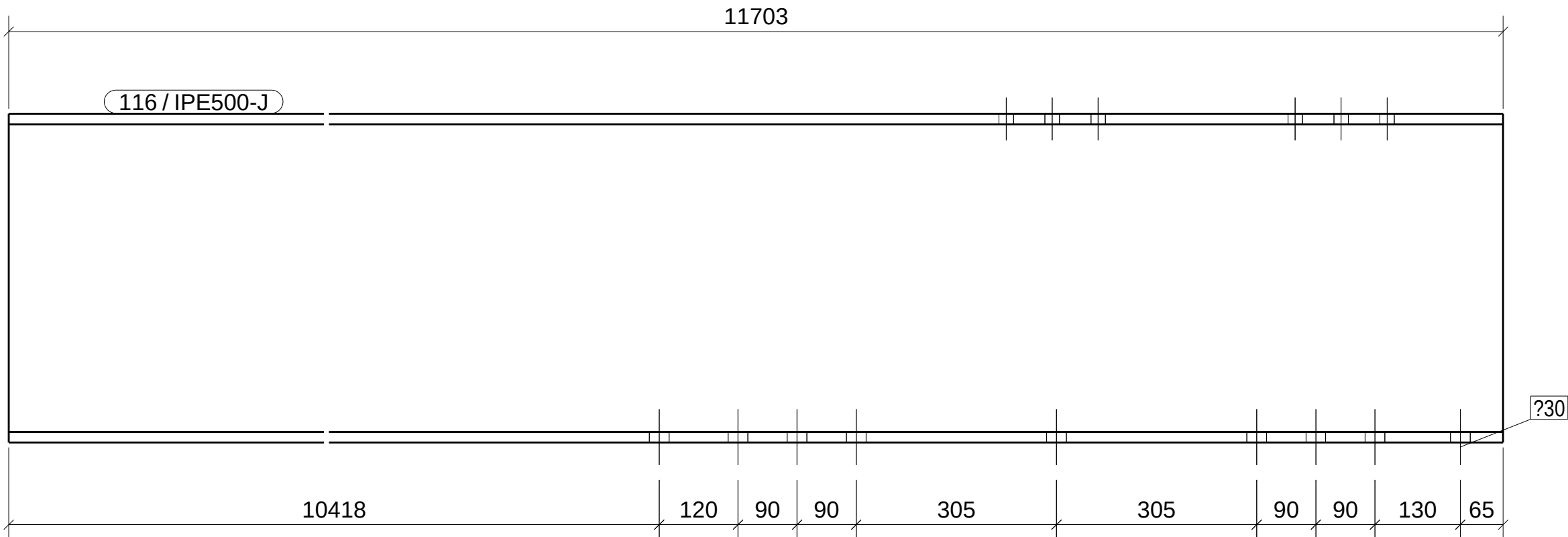
FRONT VIEW
