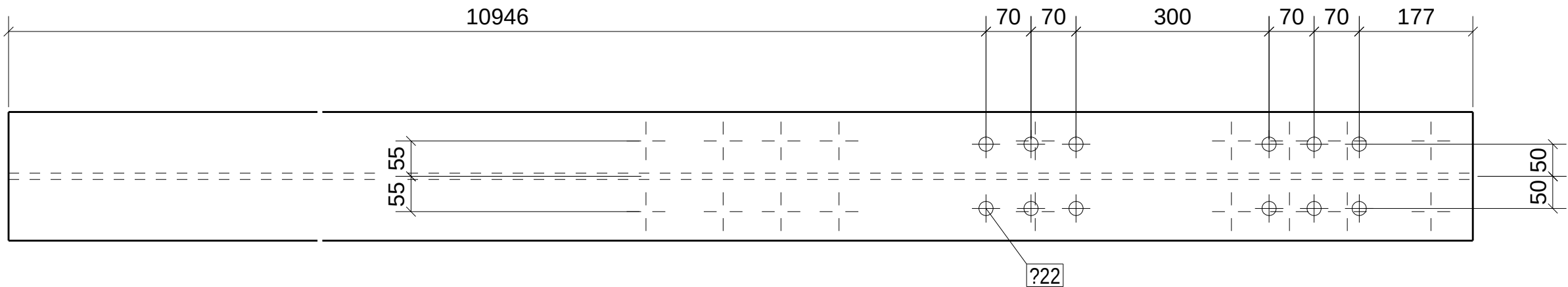
TOP VIEW
